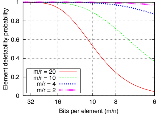
Fig. 7. Deletability estimate as function of the filter density m/n for different collision bitmap sizes r .
