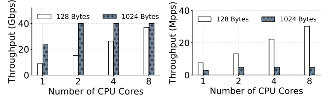
Figure 15: Performance of the buffer service showing packet processing rate and throughput scaling with the number of cores for different packet sizes.
