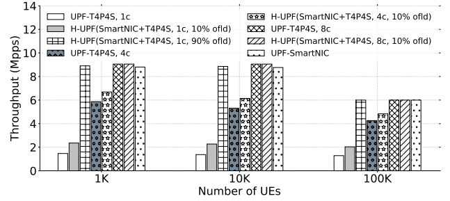
Figure 13: Performance comparison of UPF running on different targets by varying the number of UEs (c: containers, ofld: offloading, H-UPF: hybrid-UPF).
