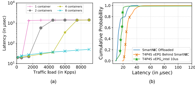
Figure 11: Latency measurements with 100K UEs and 128B packets. (a) Varying number of UPF processing containers/cores, showing UPF capacity scaling. (b) Comparison of offloaded and non-offloaded tunnels, and the imposed latency for non-offloaded traffic by the SmartNIC @ 1.5MPPS.
