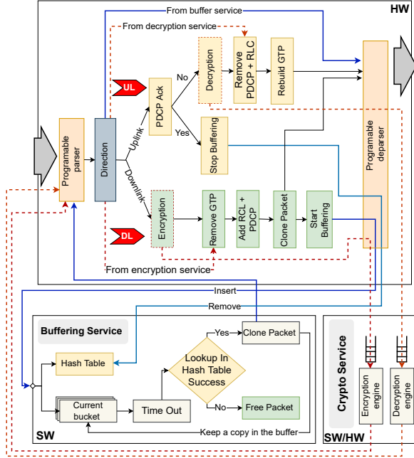
Figure 6: P4-based hybrid pipeline of the gNodeB.
