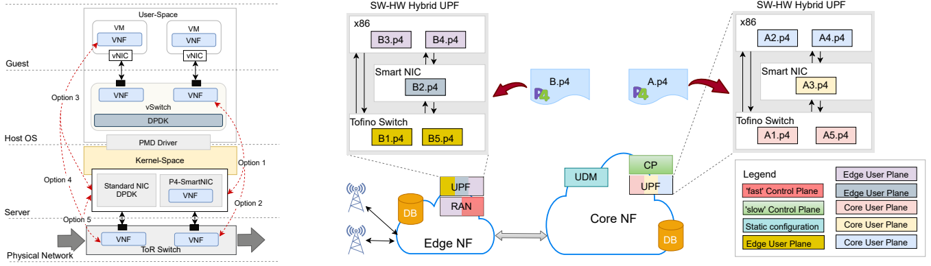
Figure 2: (Left) VNF offloading options to accelerate the packet processing path or complex/unsupported functions by P4. (Right) 5G mobile network showing the disaggregation of P4 code for UPF and gNodeB 5G functions on different targets.
