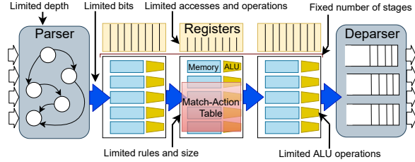
Figure 3: Resource limitations in P4 Switch ASIC.
