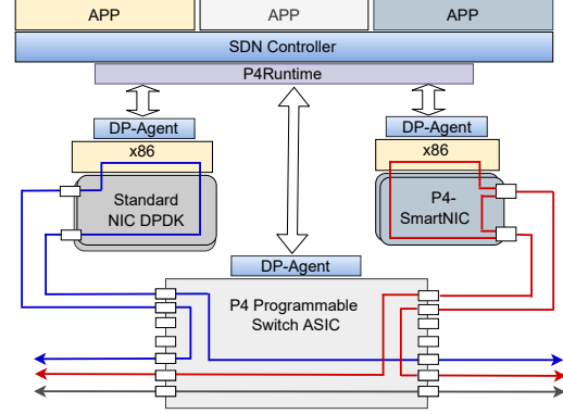
Figure 4: General architecture view of hybrid data plane
