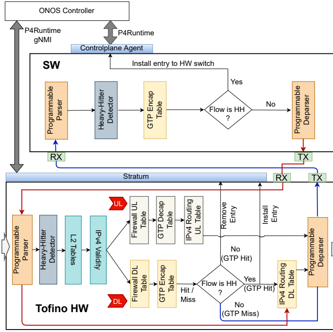
(a) P4 Based Hybrid Tofino-HW / x86
