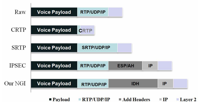
Fig 8. Overhead introduced by various protocols for a 60 bytes payload, an typical packet length for voice traffic (20ms G.729).
