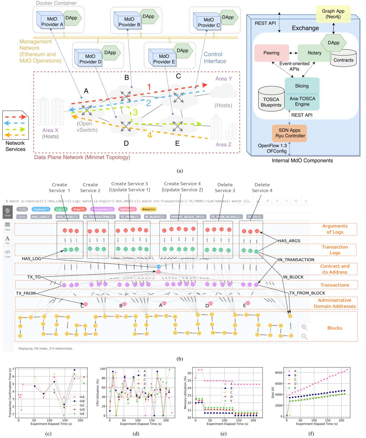
Figure 2. Experimental Setup and Overall Results. (a) Left, experimental testbed consisting of a Mininet-based topology, multi-domain orchestrators (MdO) running the DApp, and right, component details of the MdO/DApp prototype implementation. (b) Modeled Neo4j Graph of Network Service Lifecycle Events Extracted from Blockchain in Multi-domain Orchestration Experiments. (c) Transactions Confirmation Time. (d) CPU % Measurements. (e) Memory % Measurements. (f) Disk I/O Write Measurements.
