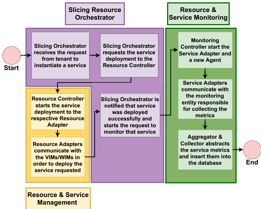
Fig. 7 The workflow responsible for deploy_service (purple-to-yellow) and start_service_monitoring (purple-to-green)
