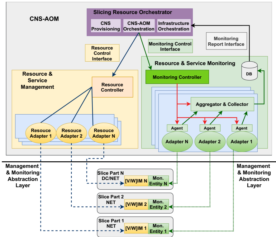
Fig. 2 CNS-AOM architecture
