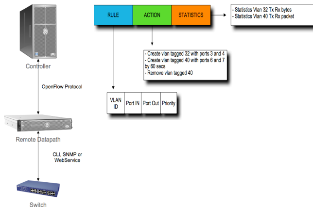
Figure 2. Overview of the virtual datapath
