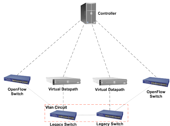
Figure 1. Openflow network is using the LegacyFlow solution.
